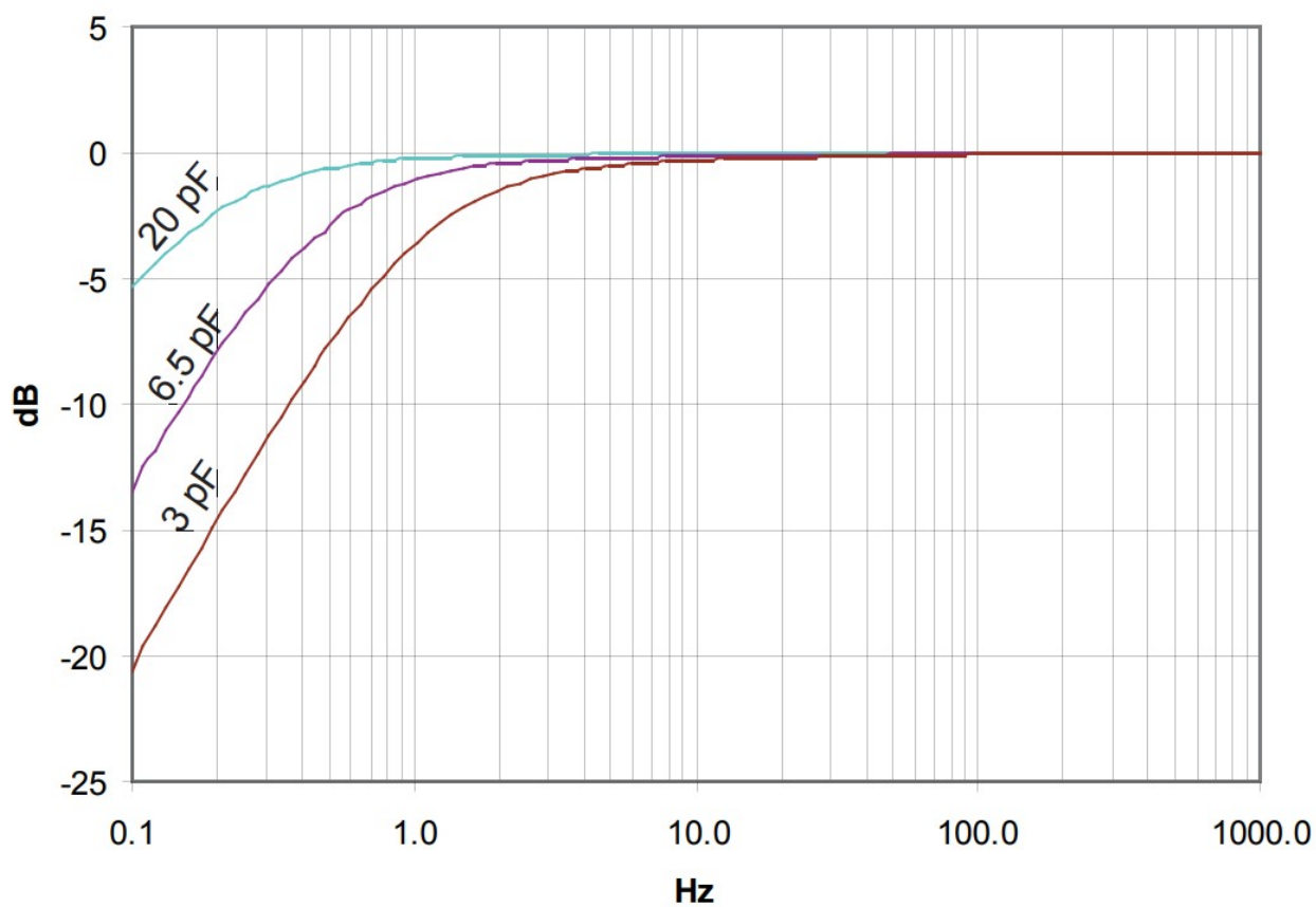
Typical frequency response for 1/2" (20 pF), 1/4" (6.5 pF) and 1/8" (3 pF) microphones
