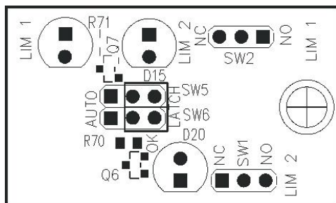
Figure 7: Auto reset
