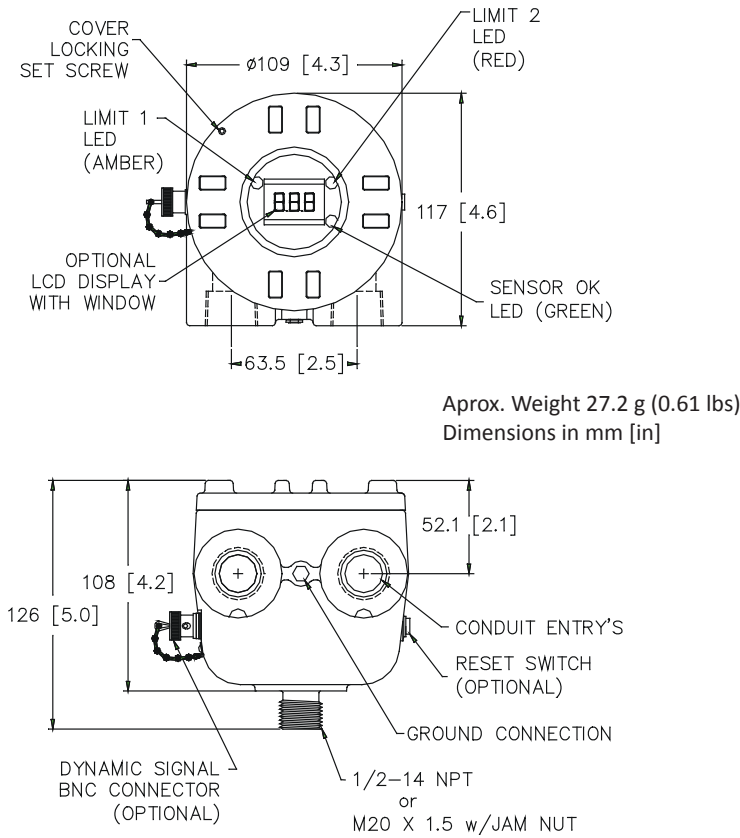
Figure 1: Housing
